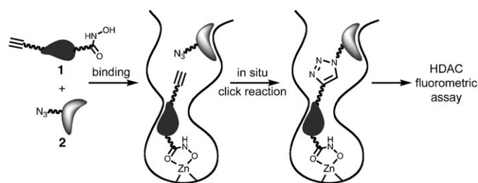
Scheme 2. In situ click chemistry screening using a fluorometric assay for HDAC activity.
