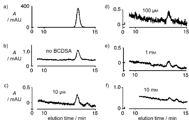
Figure 4. HPLC analysis of triazole formation from 1b (1 mM) and 2o (1 mM) in the presence of HDAC8 (0.6 μM): a) authentic sample of anti - 3 ; b) reaction in the absence of the Cu I -specific chelator BCDSA; c–f) reaction in the presence of the indicated concentration of BCDSA.
