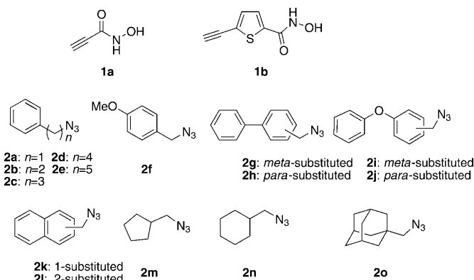
Scheme 1. Structures of alkynes 1a and 1b and azides 2a–o .
