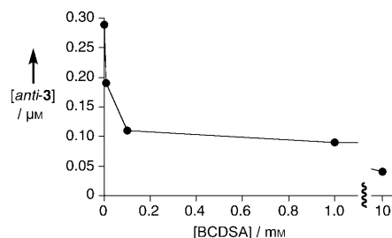
Figure 5. Inhibition of triazole anti - 3 formation by the Cu I -specific chelator BCDSA.
