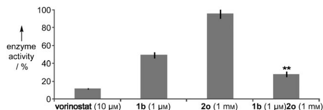
Figure 2. In situ click chemistry screening using fluorometric assay for HDAC activity. ** P < 0.01 ; ANOVA and Bonferroni-type multiple t test results indicated differences between 1b or 2o alone and a combination of 1b with 2o .
