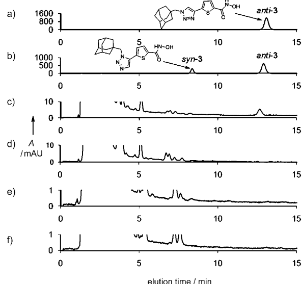
Figure 3. Identification of in situ click chemistry product generated from 1b (1 mM) and 2o (1 mM) by HPLC analysis: a) authentic sample anti - 3 (13.1 min); b) a mixture of syn - 3 (8.37 min) and anti - 3 (12.9 min); c) reaction in the presence of HDAC8 (0.6 \mu M), in situ product (12.7 min); d) reaction without enzyme; e) reaction in the presence of BSA (0.6 \mu M); f) reaction in the presence of HDAC8 (0.6 \mu M) and vorinostat (10 mM). mAU = milli absorbance units.
