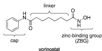
Figure 1. Structural characteristics of HDAC inhibitors.
